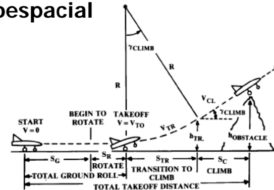
Fig. 17.17 Takeoff analysis.
