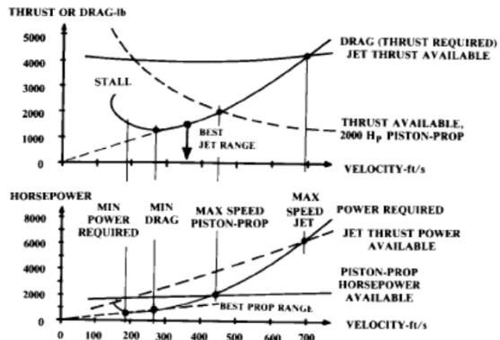
Fig. 17.2 Thrust and power.
