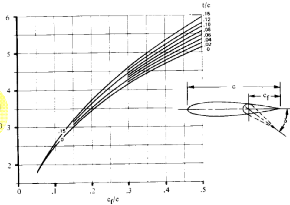
Fig. 16.6 Theoretical lift increment for plain flaps. (Ref. 37)
