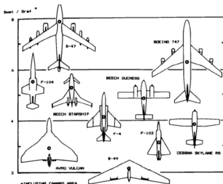
Fig. 3.5 Wetted area ratios.
