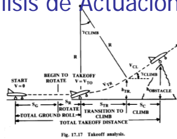
Fig. 17.17 Takeoff analysis.
